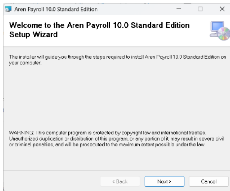
Figure 1.1: Setup Wizard
